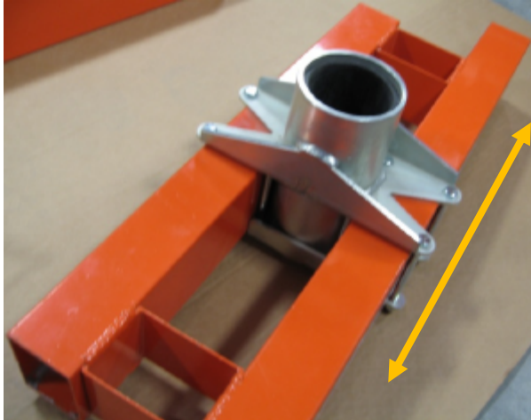
Figure 8, Assembled Base Frame / Sleeve (Pro-3 HD is Similar)
