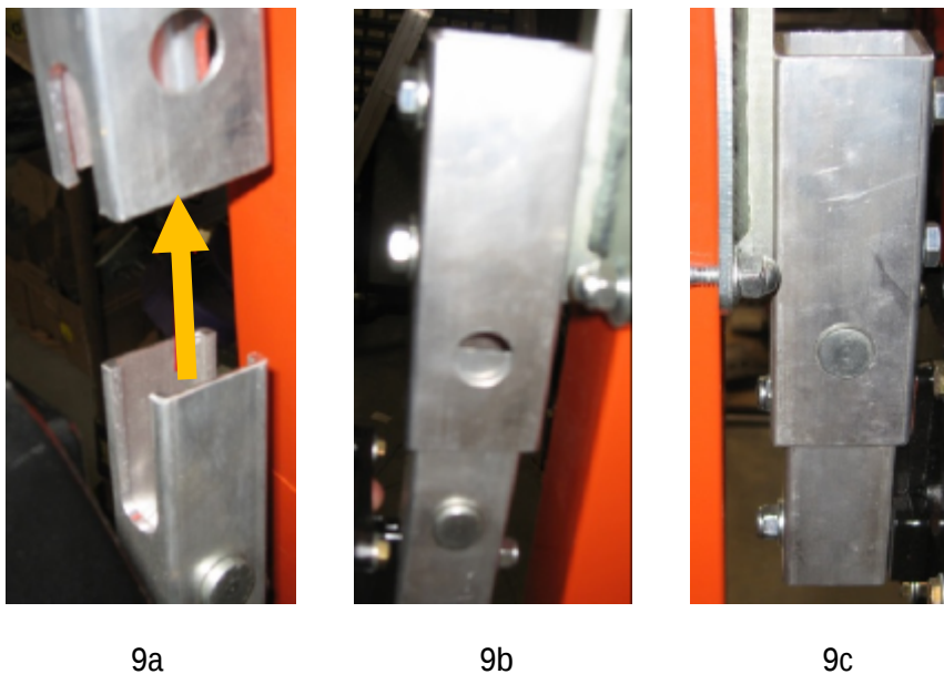
Figure 9, Tuff Built Products Winch / SRL Installation.
