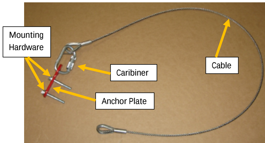
Figure 11, Optional SRL Mounting Anchor Cable Kit
