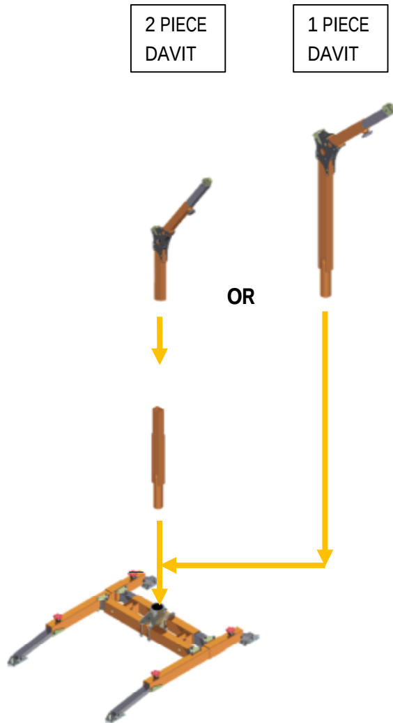
Figure 8, Installation of Pro-I Davit Arm to Pro-III Series Mounting Base (Pro-3 HD is Similar)
