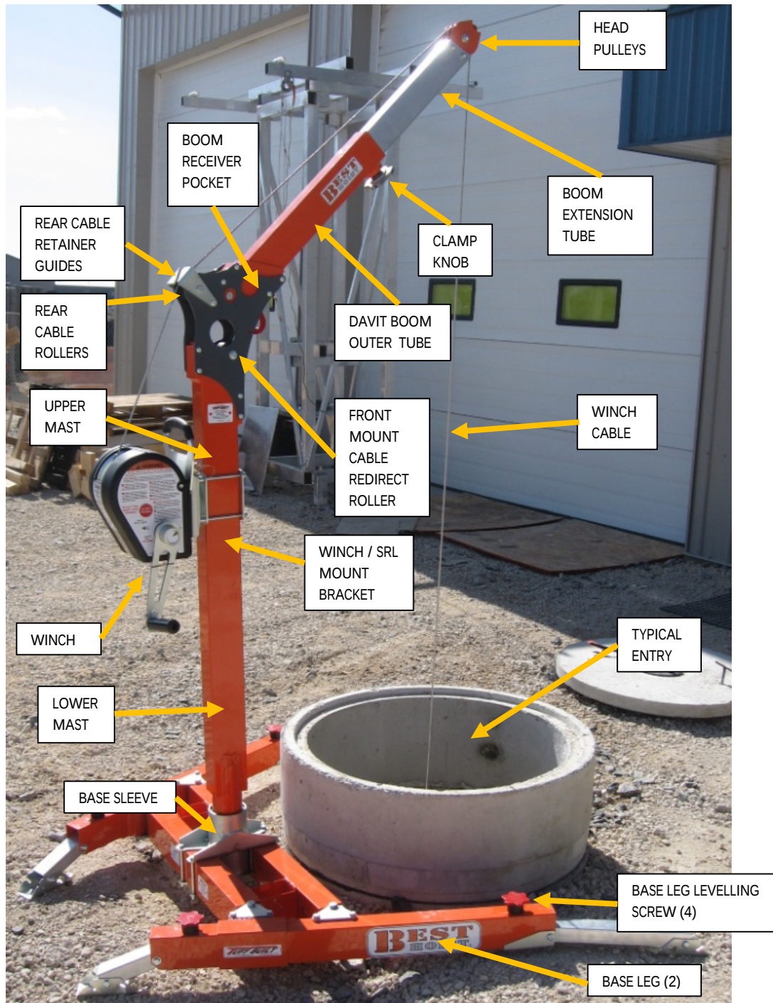
Figure 1, Pro-3 Davit System Parts and Location (Pro-3 HD is Similar)
