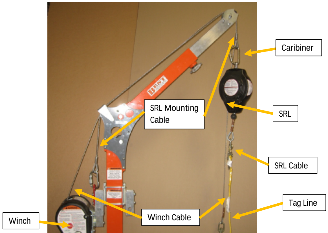
Figure 10, Optional SRL Mounting Anchor Cable Installation
